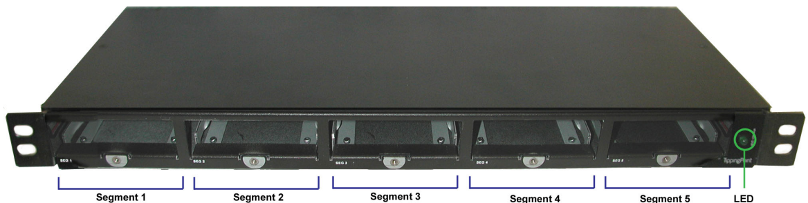
Figure 2-3 Modular ZPHA device front panel (without segments)
